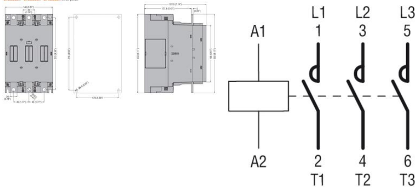
BF2000E... - BF3000E... - BF4000E... three poles
