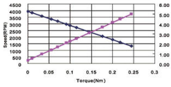
MB054TP100 CURVE
