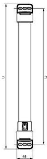
LED 021 (Size 1) L1 = 400 mm L2 = 375 mm
