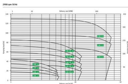
CHARACTERISTIC MAPS
