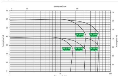
CHARACTERISTIC MAPS
