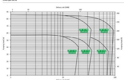
CHARACTERISTIC MAPS
