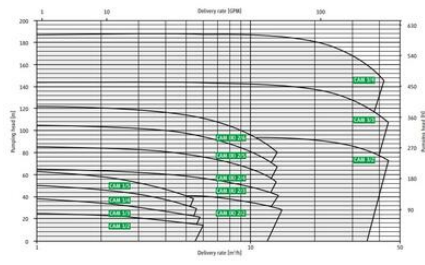
3500 rpm 60 Hz
