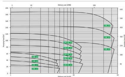
CHARACTERISTIC MAPS
