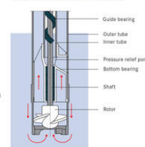
F 314/PP 314 - The small sealless drum pump
