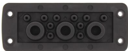
KES 13/24 10x Ø3.2 - 6.3mm 3x Ø16 - 20.5mm
